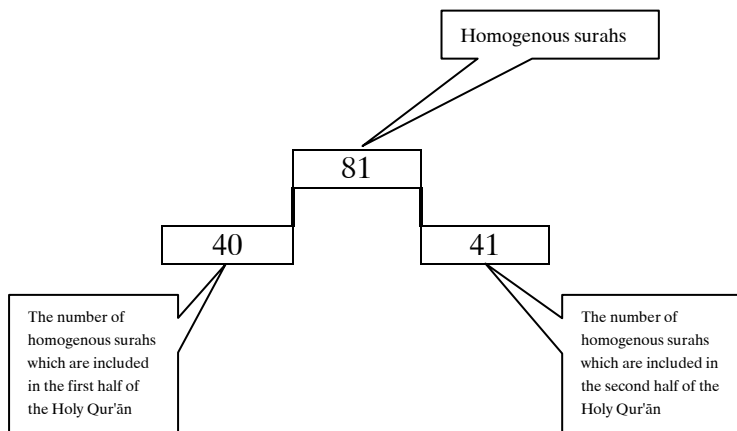
Figure-16 Distribution of the homogeneous surahs (as prime and non-prime) is shown.
