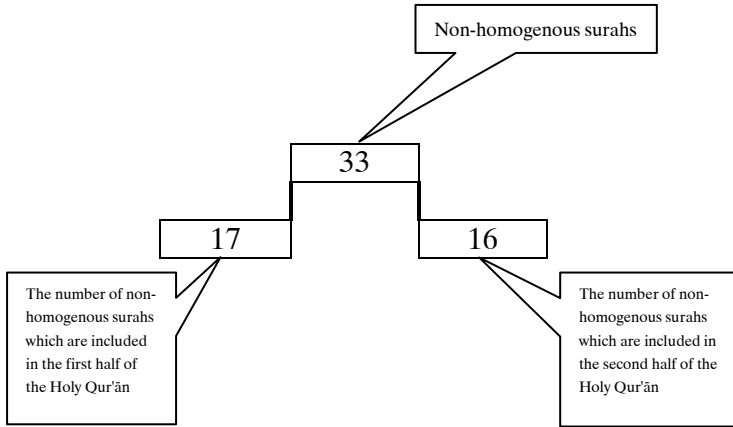
Figure-17 Distribution of the non-homogeneous surahs (as prime and non-prime) is shown.
